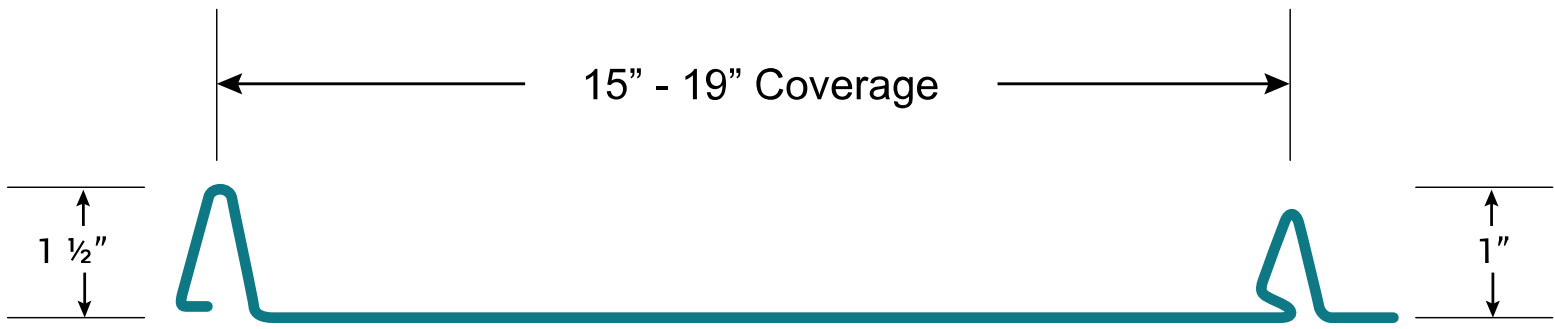
Panel Profile
