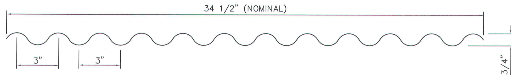
PANEL PROFILE
