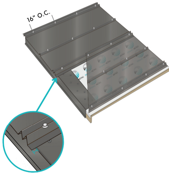
PANEL OVERHANG 1-1/2" MAXIMUM
