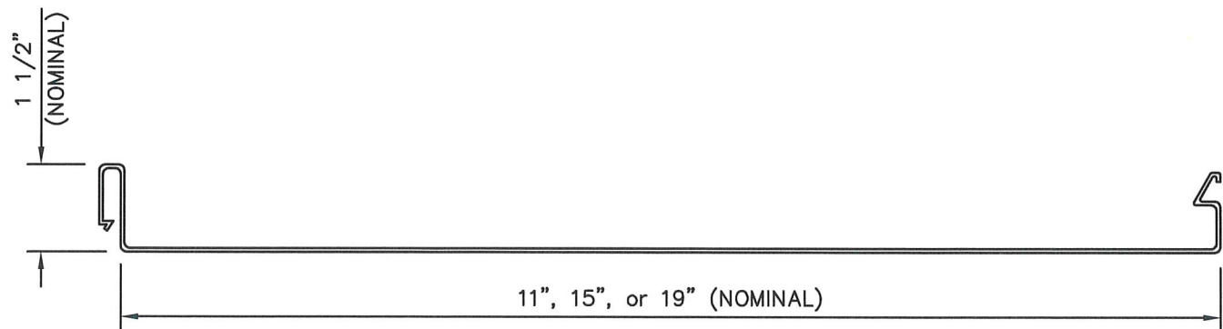
PANEL PROFILE
