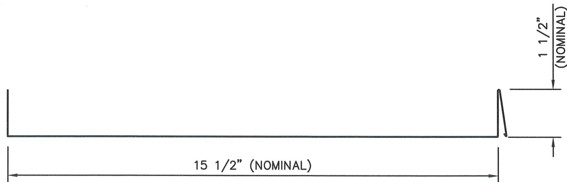
PANEL PROFILE
