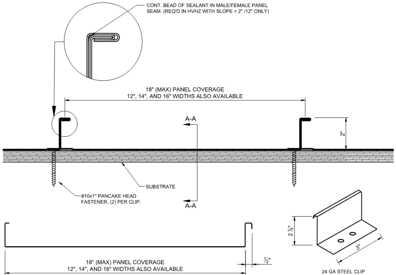
PANEL PROFILE
