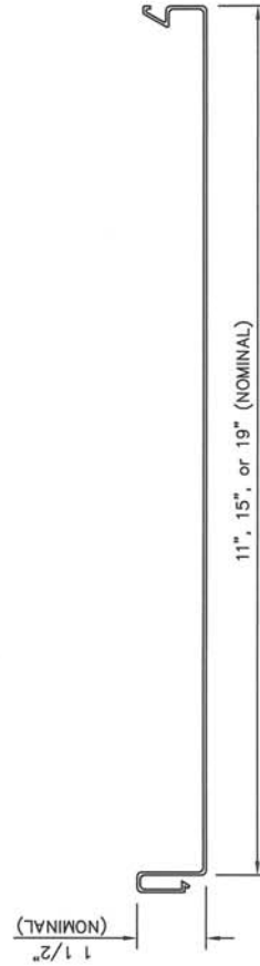
PANEL PROFILE
