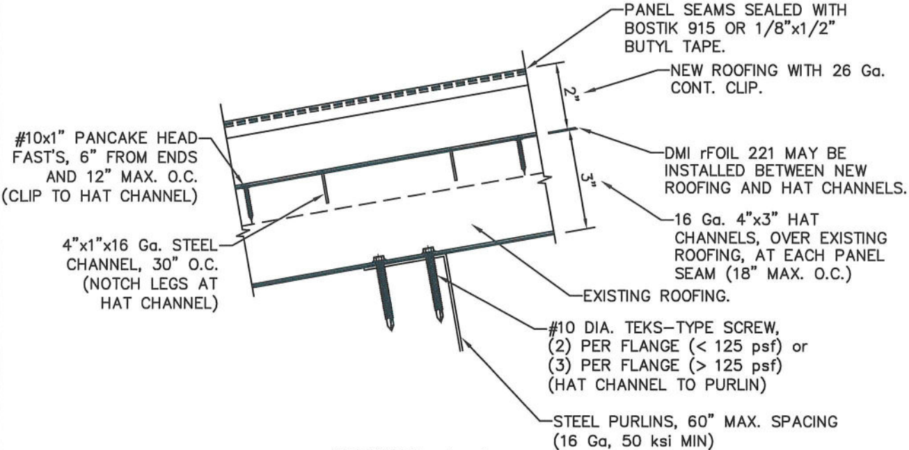
SECTION A-A (WITH EXISTING ROOFING)
